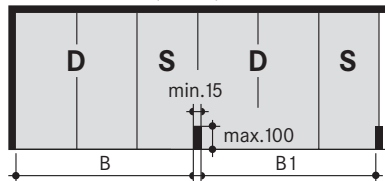
Combinated unit (6 Pkw)
