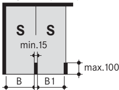
Single unit (2 Pkw)
